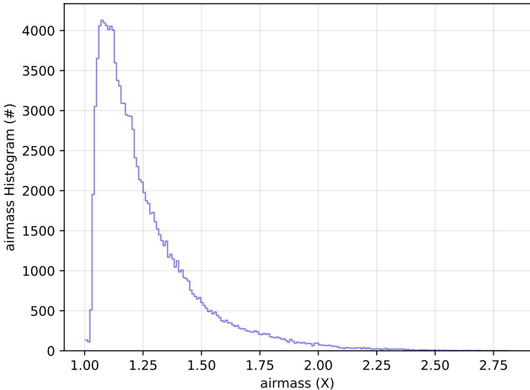
too_elab_r256_d2_ugrizy_v3.4_10yrs WFD u band: airmass Histogram
