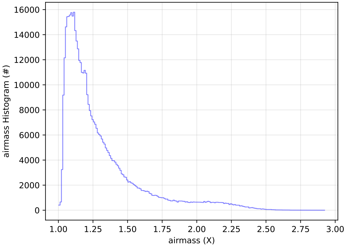
too_elab_r256_d2_ugrizy_v3.4_10yrs WFD r band: airmass Histogram
