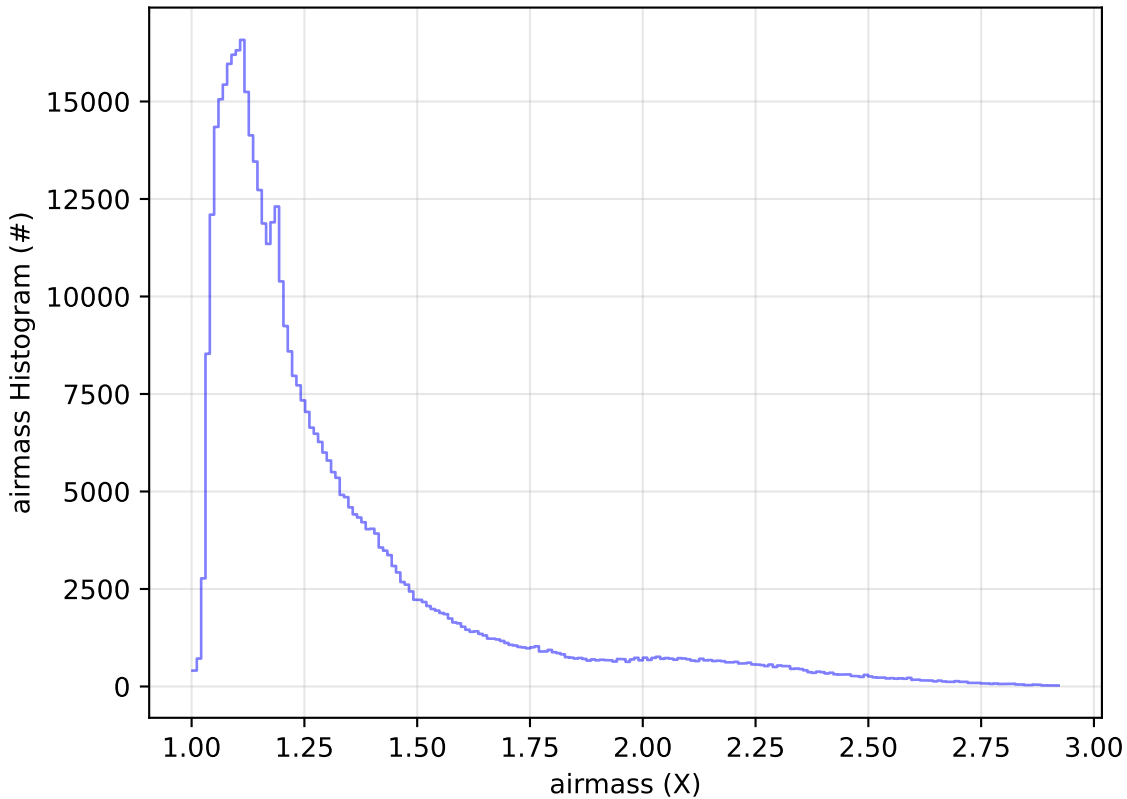
too_elab_r256_d2_ugrizy_v3.4_10yrs WFD i band: airmass Histogram
