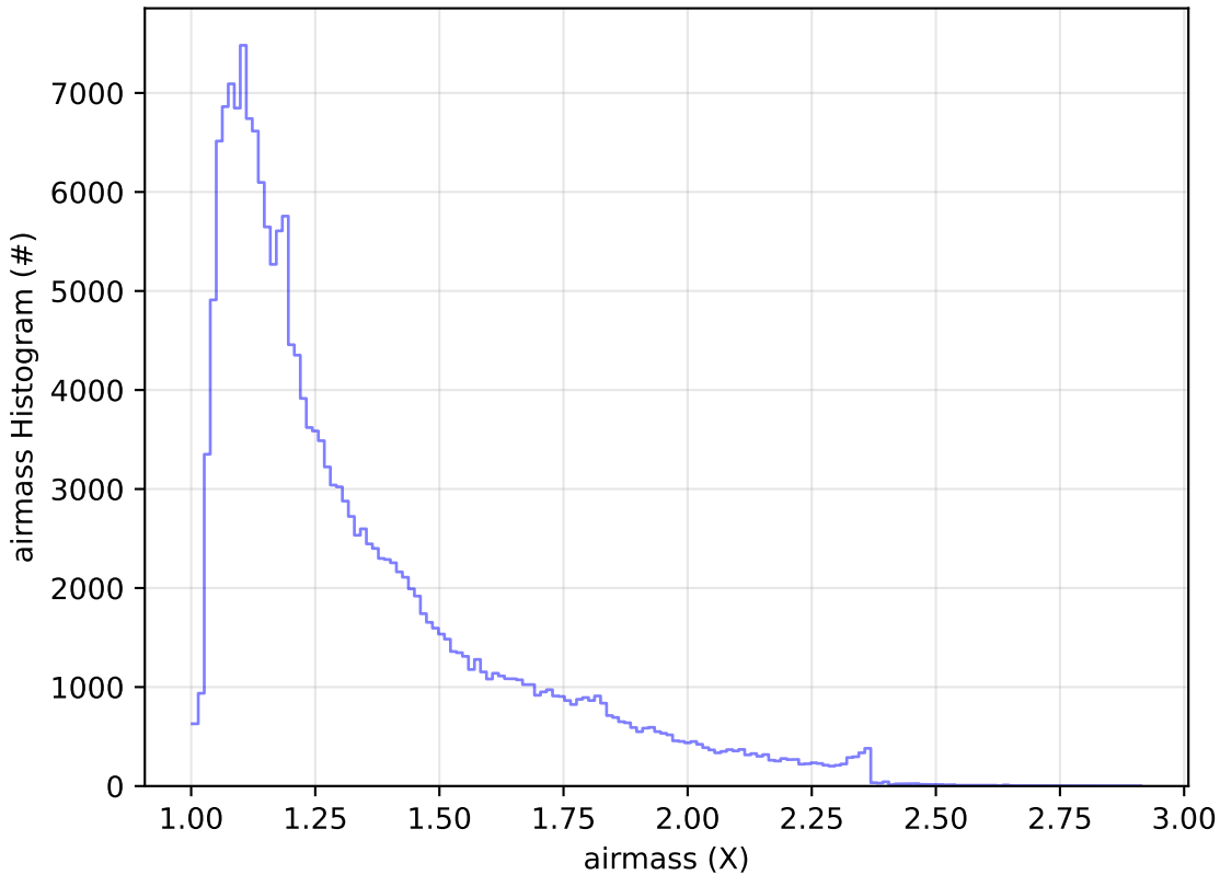
too_elab_r256_d2_ugrizy_v3.4_10yrs WFD g band: airmass Histogram
