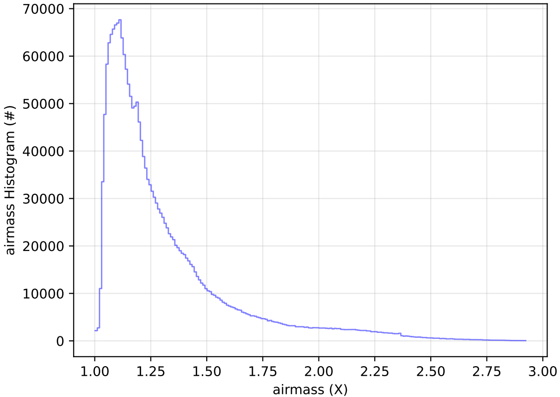
too_elab_r256_d2_ugrizy_v3.4_10yrs WFD all bands: airmass Histogram
