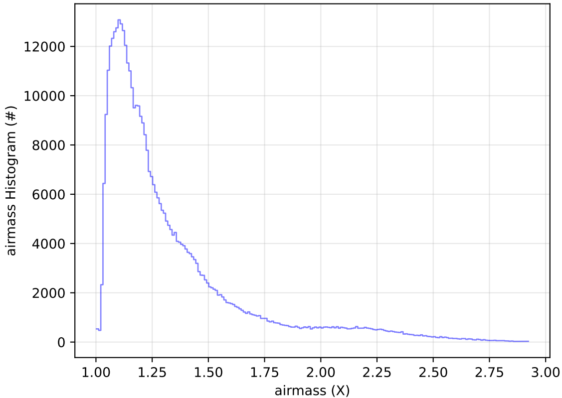
too_elab_r256_d2_ugrizy_v3.4_10yrs All sky z band: airmass Histogram
