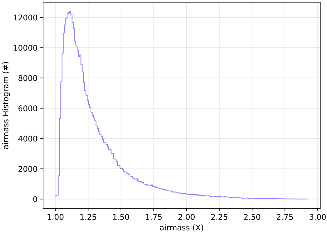
too_elab_r256_d2_ugrizy_v3.4_10yrs All sky y band: airmass Histogram
