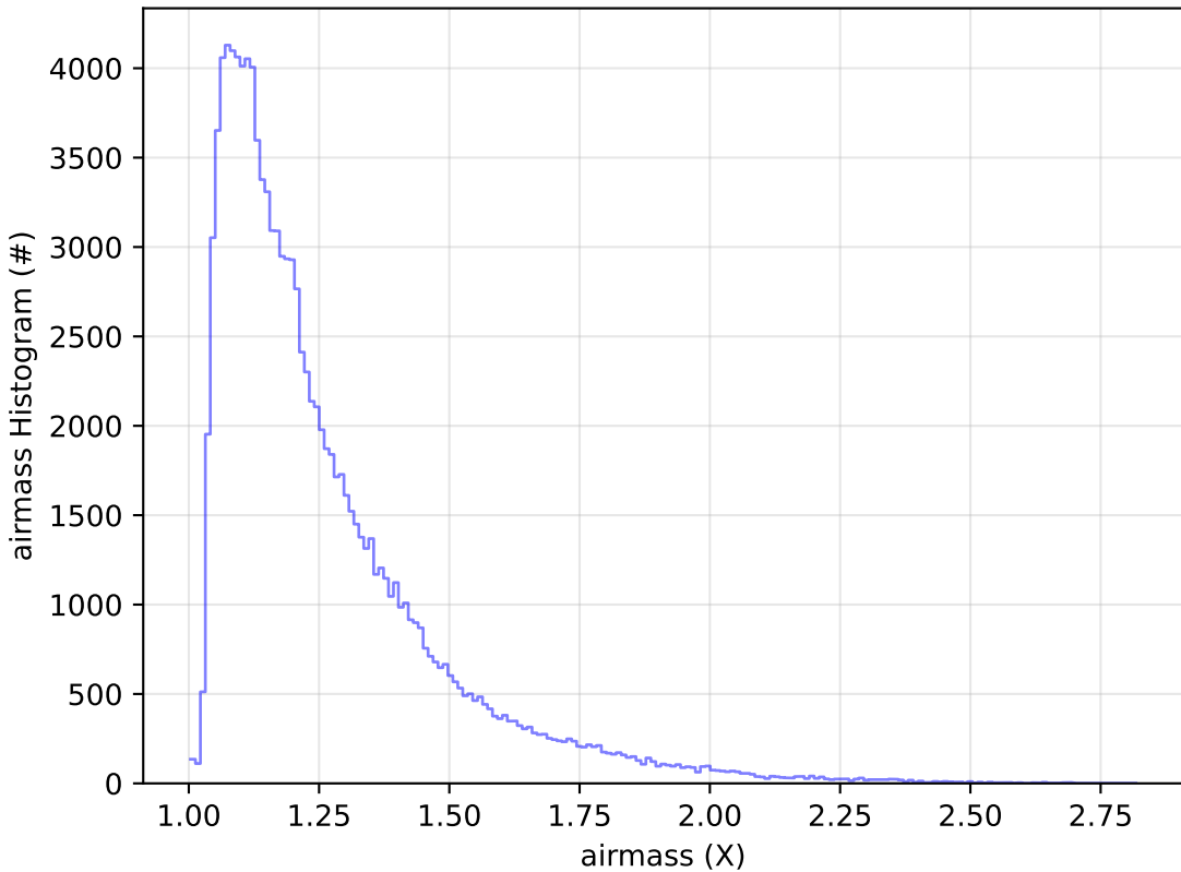
too_elab_r256_d2_ugrizy_v3.4_10yrs All sky u band: airmass Histogram
