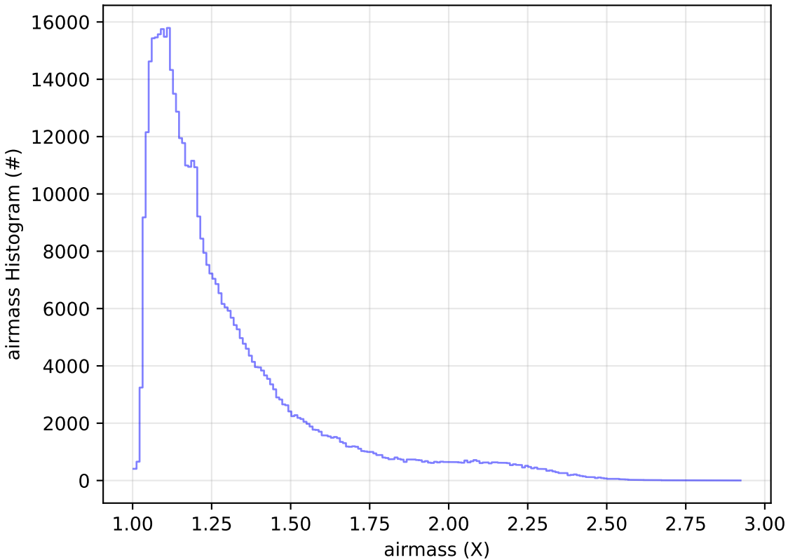
too_elab_r256_d2_ugrizy_v3.4_10yrs All sky r band: airmass Histogram
