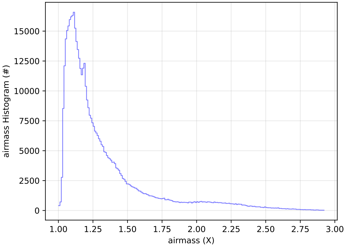
too_elab_r256_d2_ugrizy_v3.4_10yrs All sky i band: airmass Histogram
