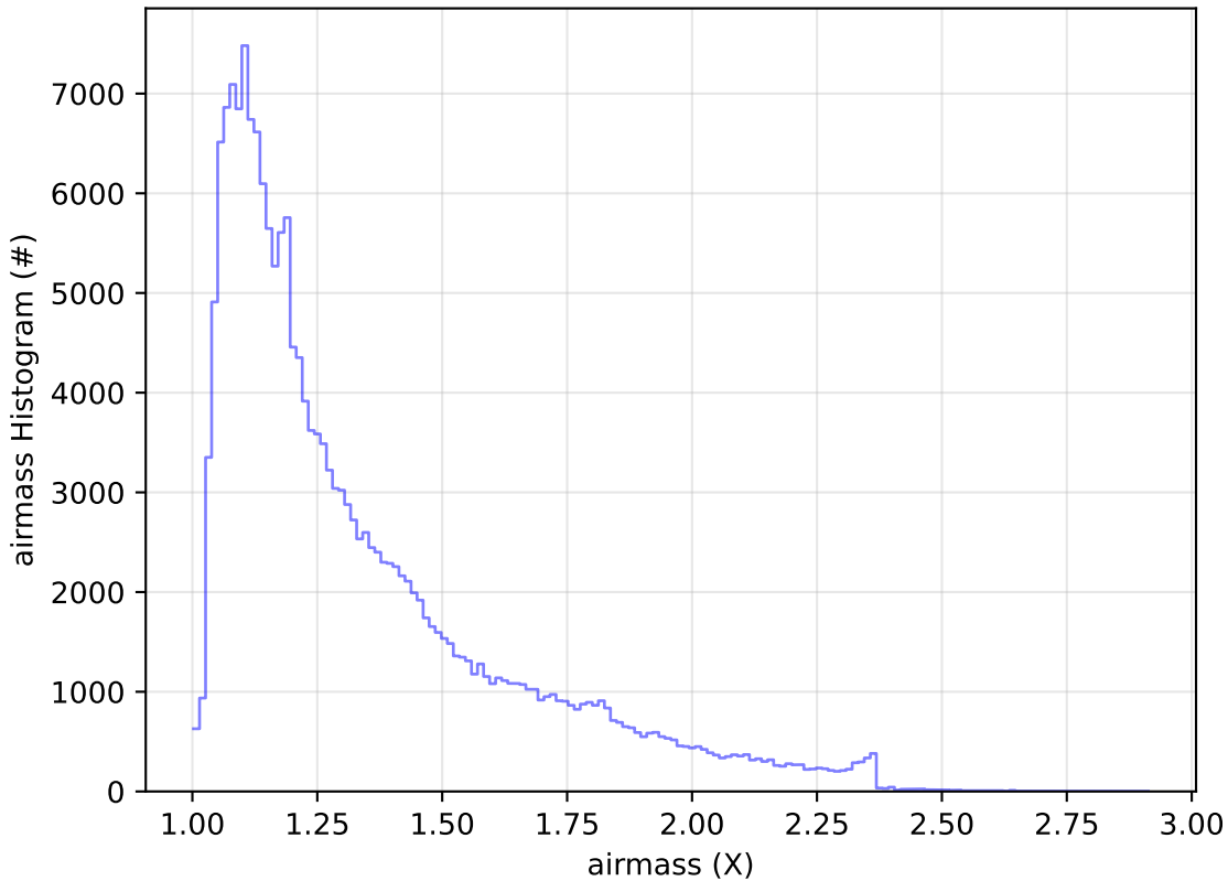
too_elab_r256_d2_ugrizy_v3.4_10yrs All sky g band: airmass Histogram
