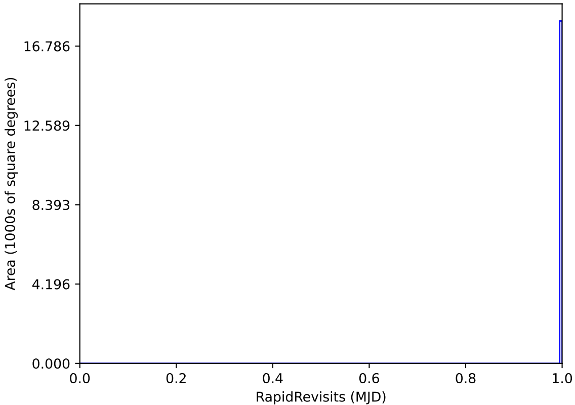
too_elab_r256_d2_ugrizy_v3.4_10yrs WFD: RapidRevisits
