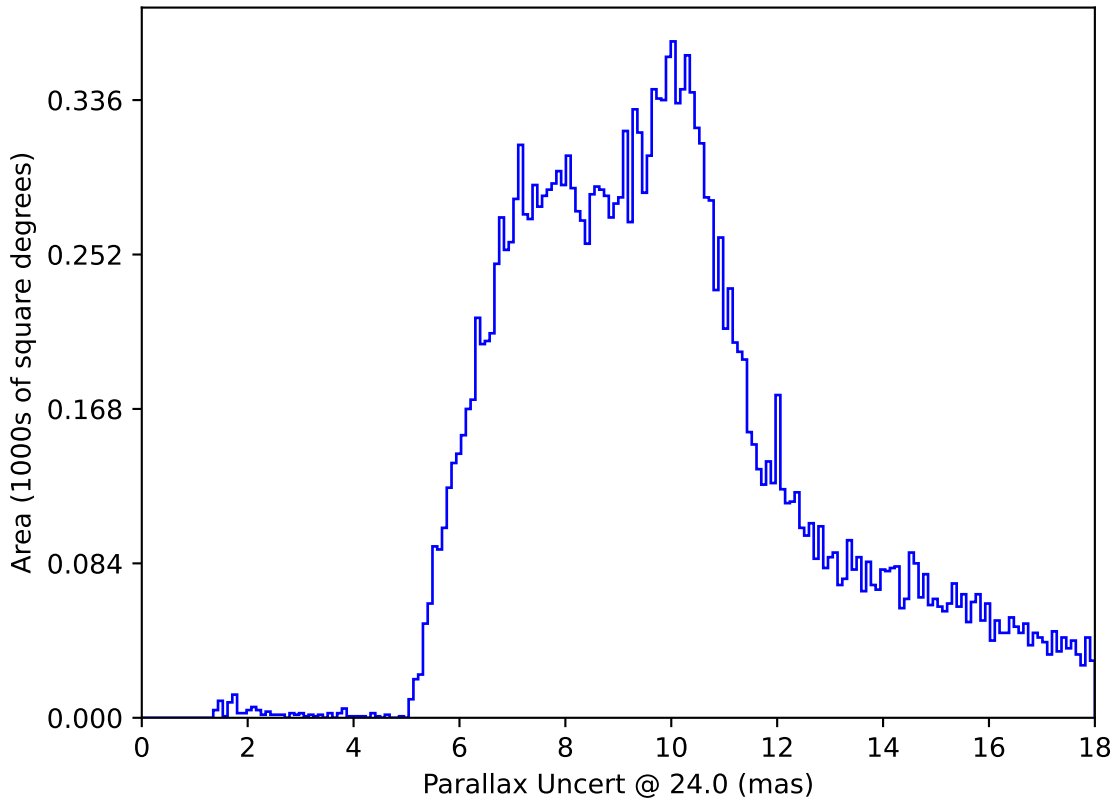
too_elab_r256_d2_ugrizy_v3.4_10yrs All sky: Parallax Uncert @ 24.0
