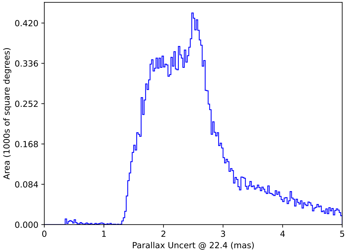
too_elab_r256_d2_ugrizy_v3.4_10yrs All sky: Parallax Uncert @ 22.4
