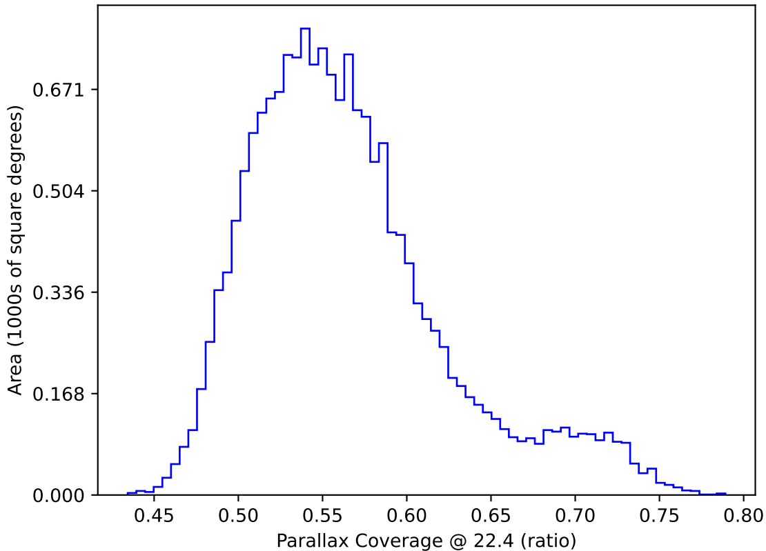
too_elab_r256_d2_ugrizy_v3.4_10yrs WFD: Parallax Coverage @ 22.4
