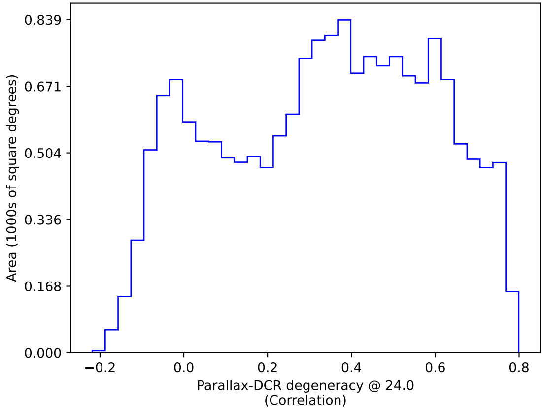
too_elab_r256_d2_ugrizy_v3.4_10yrs WFD: Parallax-DCR degeneracy @ 24.0
