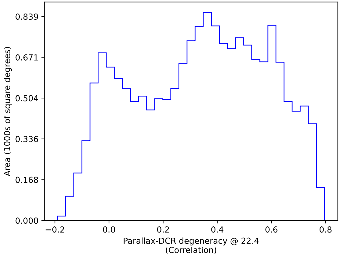
too_elab_r256_d2_ugrizy_v3.4_10yrs WFD: Parallax-DCR degeneracy @ 22.4
