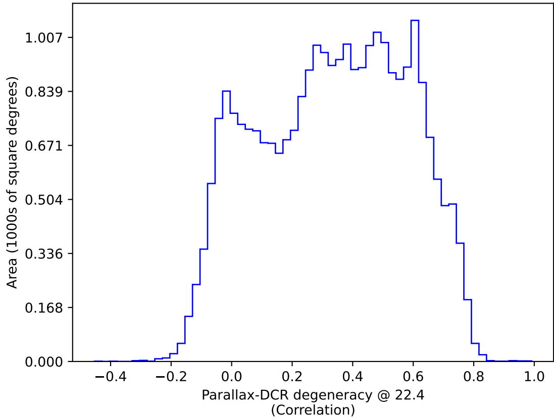
too_elab_r256_d2_ugrizy_v3.4_10yrs All sky: Parallax-DCR degeneracy @ 22.4
