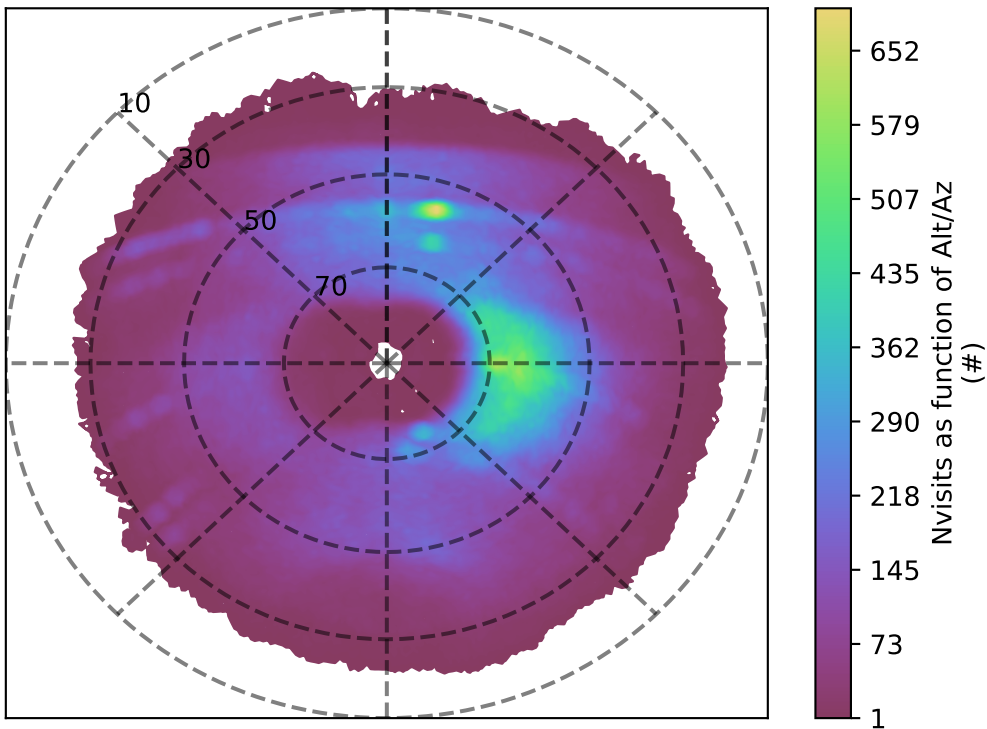
too_elab_r256_d2_ugrizy_v3.4_10yrs u band: Nvisits as function of Alt/Az
