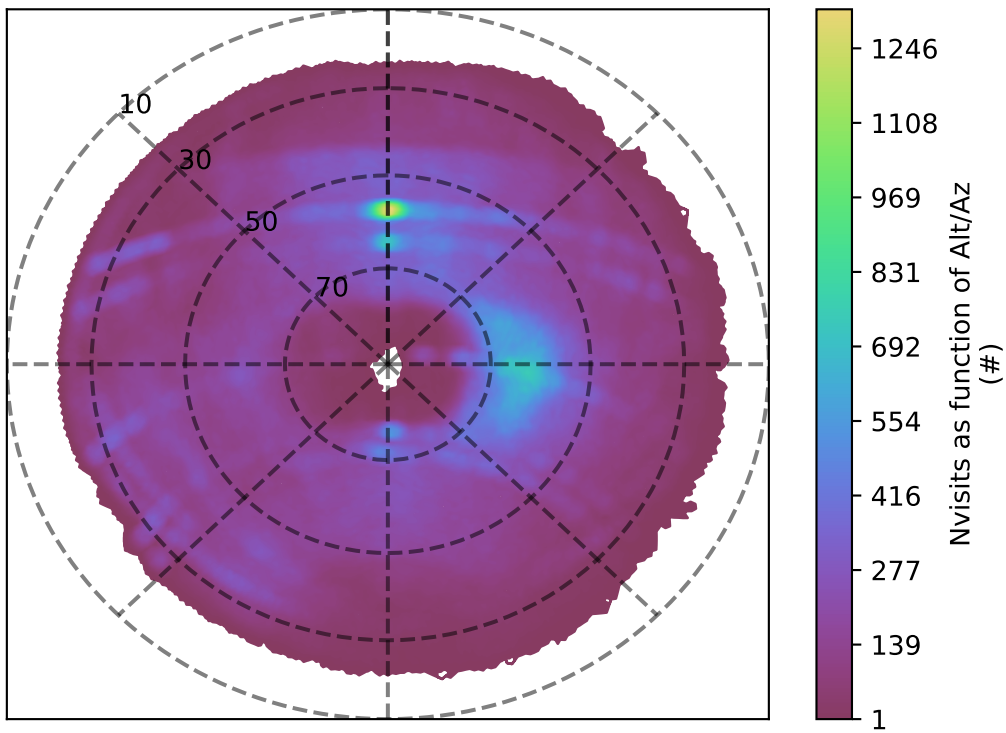
too_elab_r256_d2_ugrizy_v3.4_10yrs g band: Nvisits as function of Alt/Az
