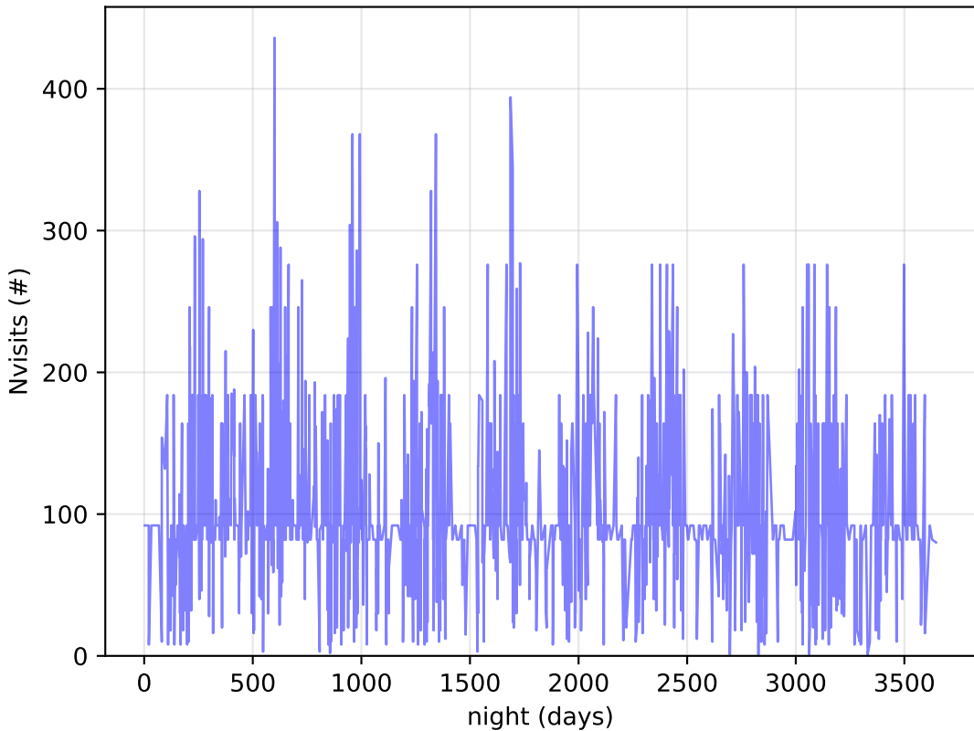
too_elab_r256_d2_ugrizy_v3.4_10yrs DDF: Nvisits
