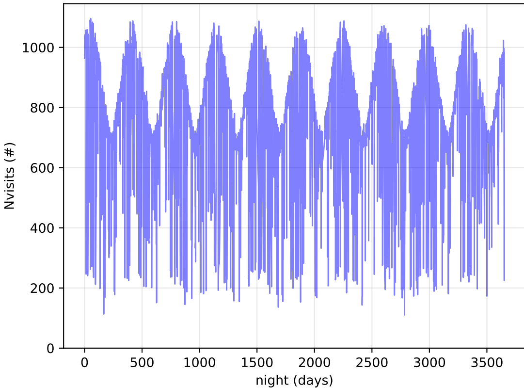
too_elab_r256_d2_ugrizy_v3.4_10yrs All visits: Nvisits
