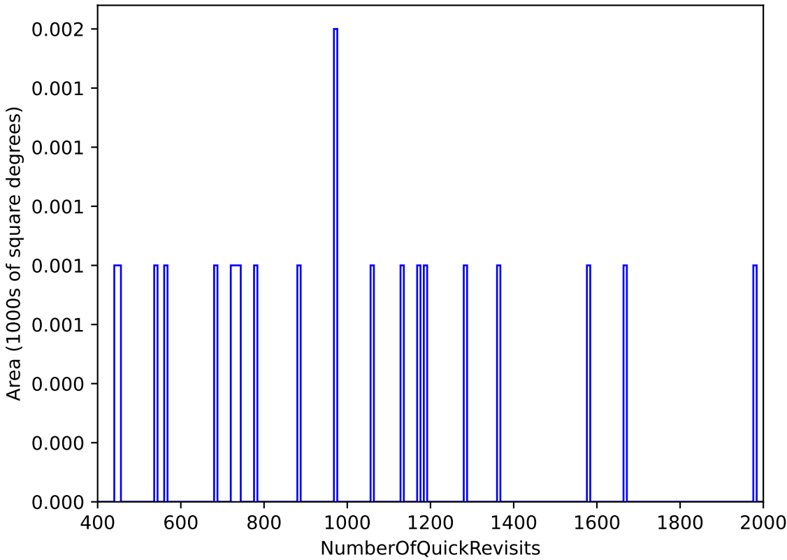
too_elab_r256_d2_ugrizy_v3.4_10yrs All sky: NumberOfQuickRevisits
