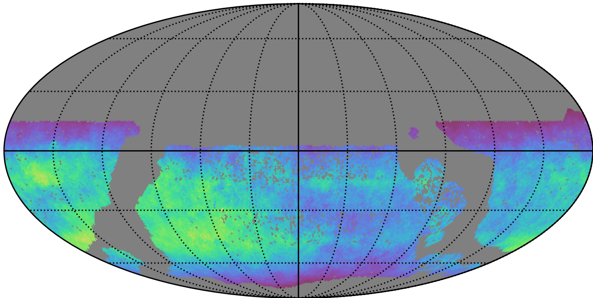
too_elab_r256_d2_ugrizy_v3.4_10yrs WFD z band: Normalized Teff
