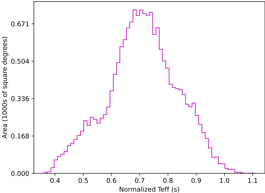
too_elab_r256_d2_ugrizy_v3.4_10yrs WFD z band: Normalized Teff
