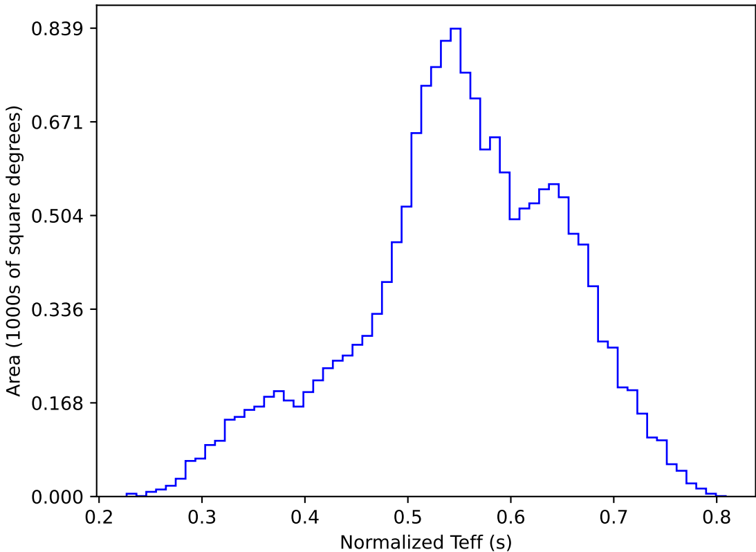
too_elab_r256_d2_ugrizy_v3.4_10yrs WFD y band: Normalized Teff
