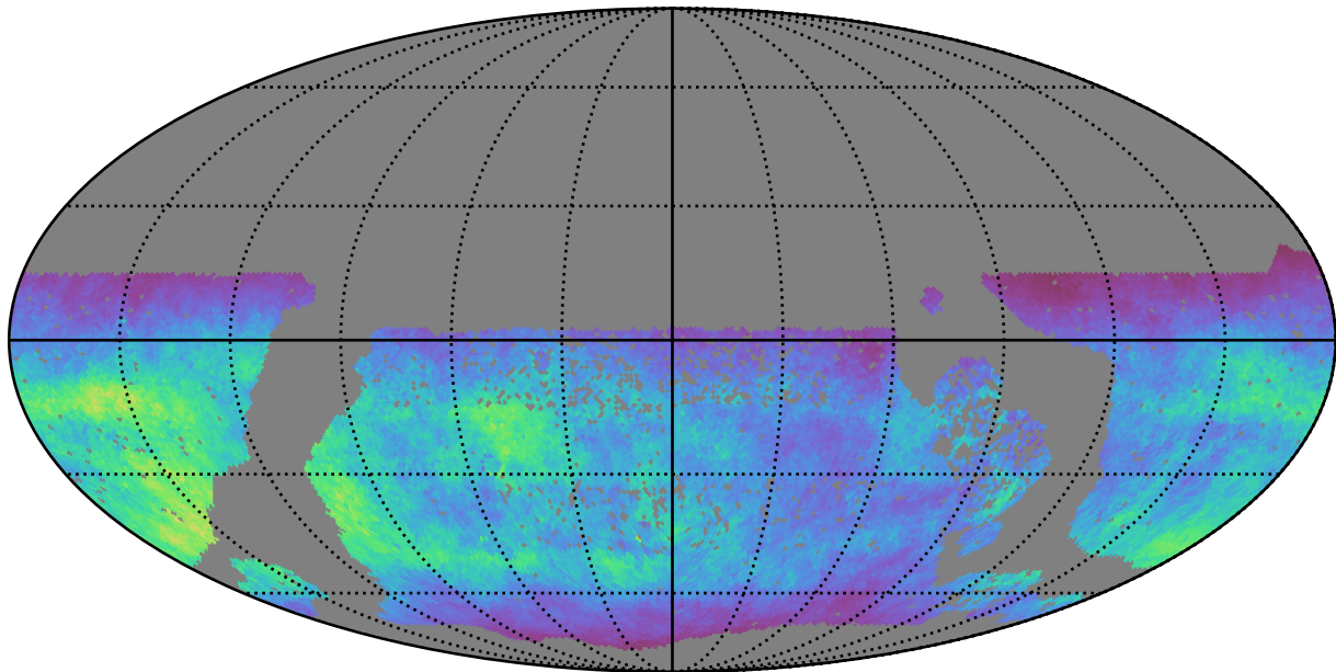
too_elab_r256_d2_ugrizy_v3.4_10yrs WFD u band: Normalized Teff
