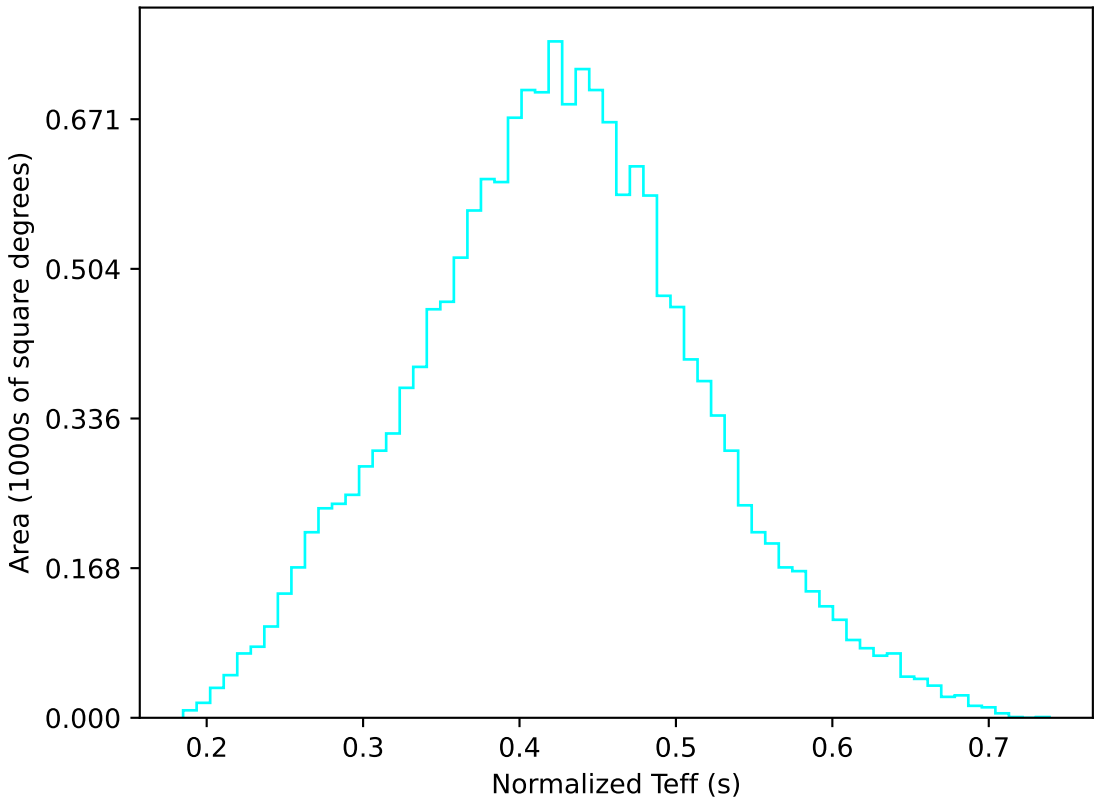
too_elab_r256_d2_ugrizy_v3.4_10yrs WFD u band: Normalized Teff
