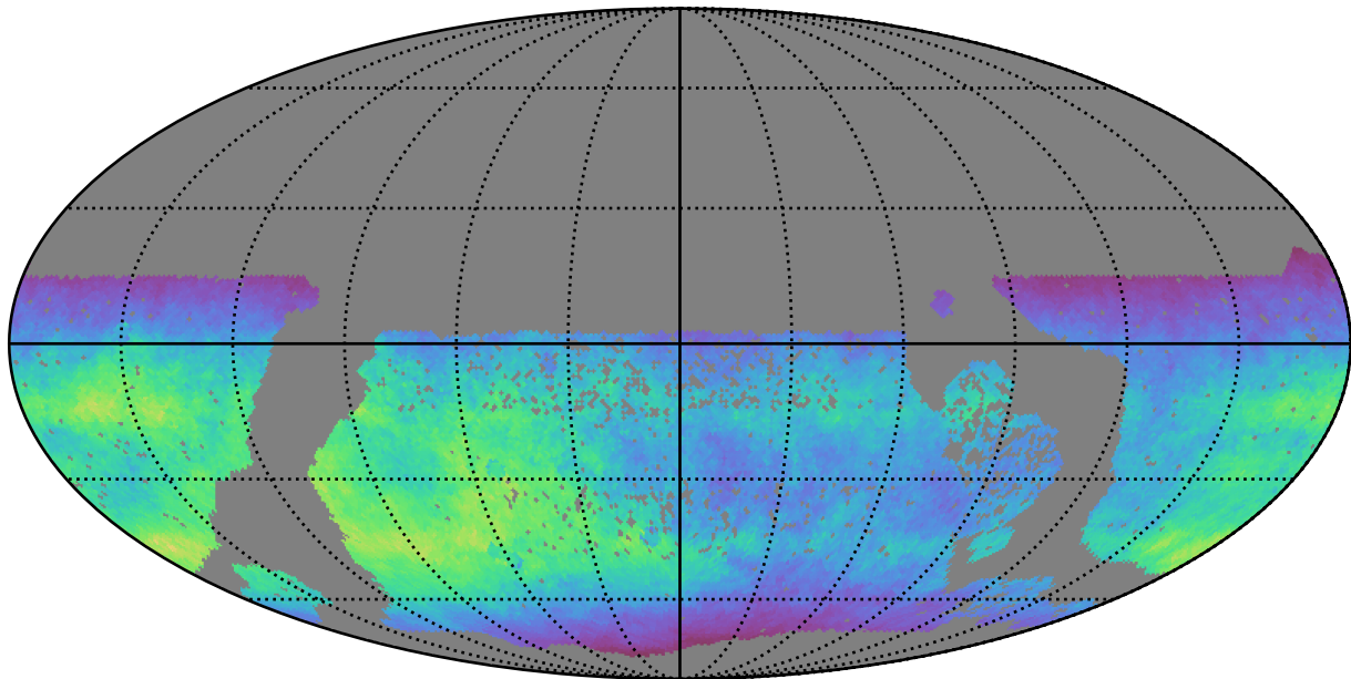
too_elab_r256_d2_ugrizy_v3.4_10yrs WFD i band: Normalized Teff
