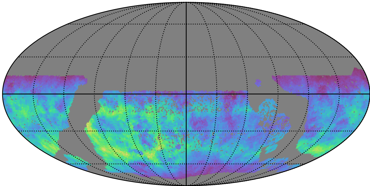
too_elab_r256_d2_ugrizy_v3.4_10yrs WFD g band: Normalized Teff
