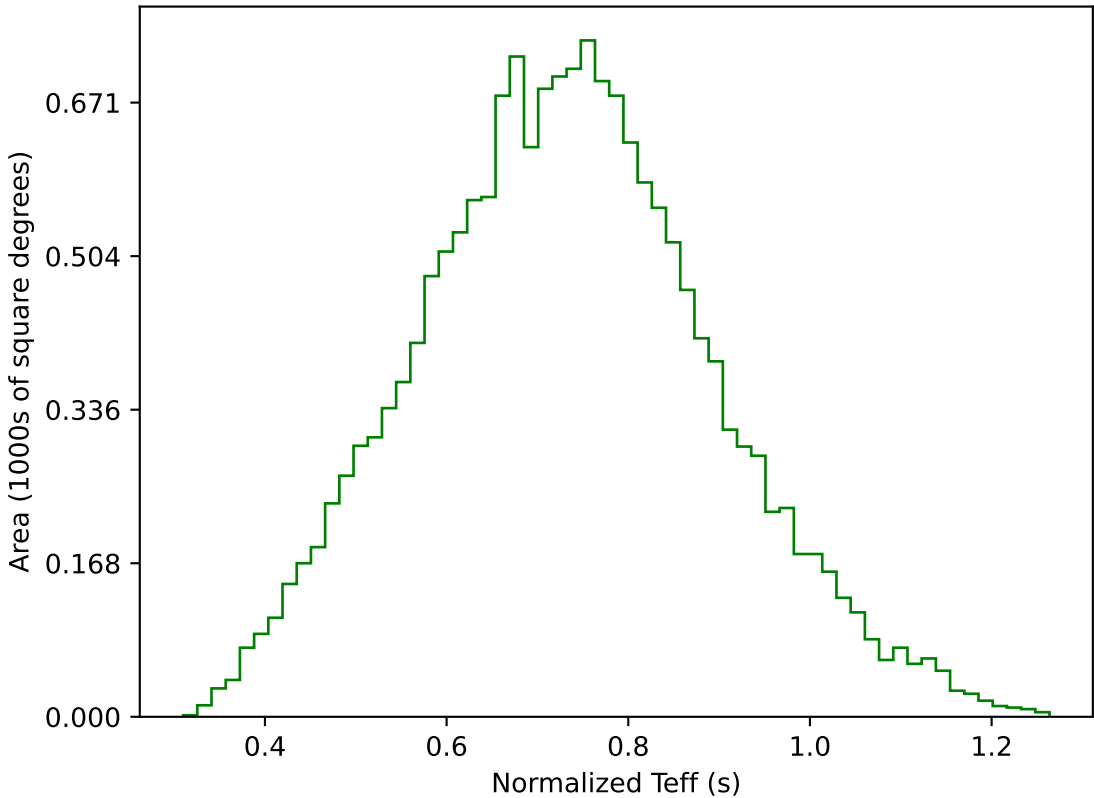
too_elab_r256_d2_ugrizy_v3.4_10yrs WFD g band: Normalized Teff
