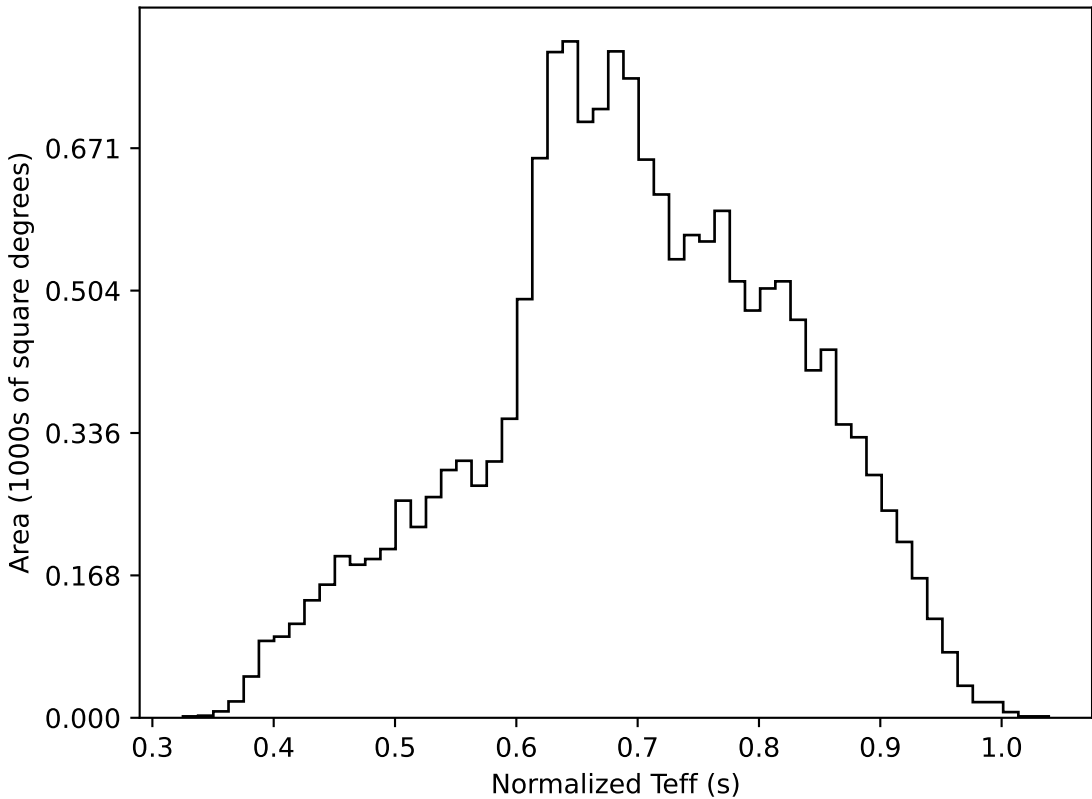
too_elab_r256_d2_ugrizy_v3.4_10yrs WFD all bands: Normalized Teff
