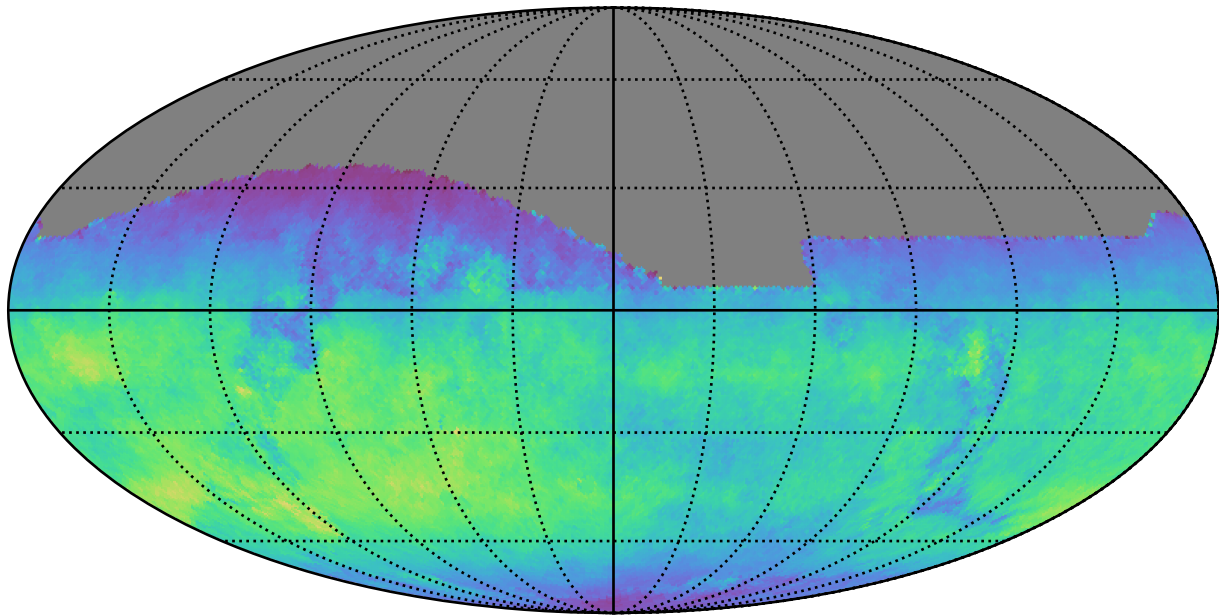
too_elab_r256_d2_ugrizy_v3.4_10yrs All sky z band: Normalized Teff
