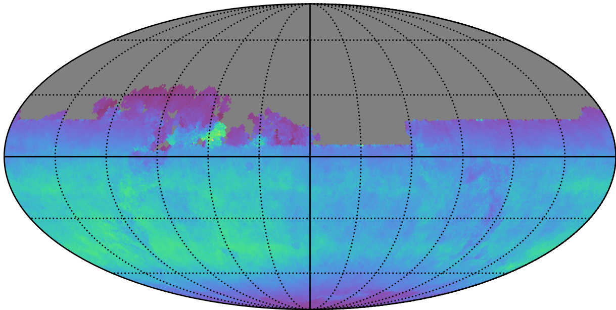
too_elab_r256_d2_ugrizy_v3.4_10yrs All sky y band: Normalized Teff
