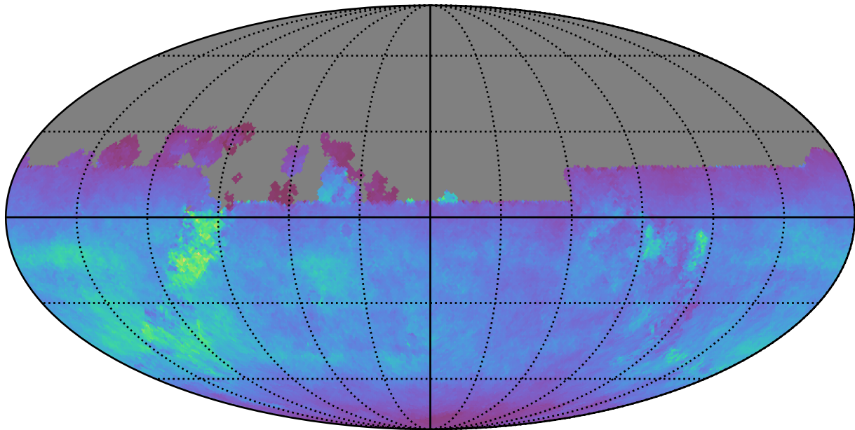
too_elab_r256_d2_ugrizy_v3.4_10yrs All sky u band: Normalized Teff
