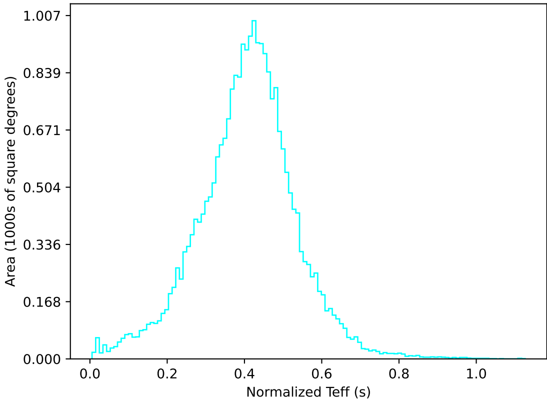
too_elab_r256_d2_ugrizy_v3.4_10yrs All sky u band: Normalized Teff
