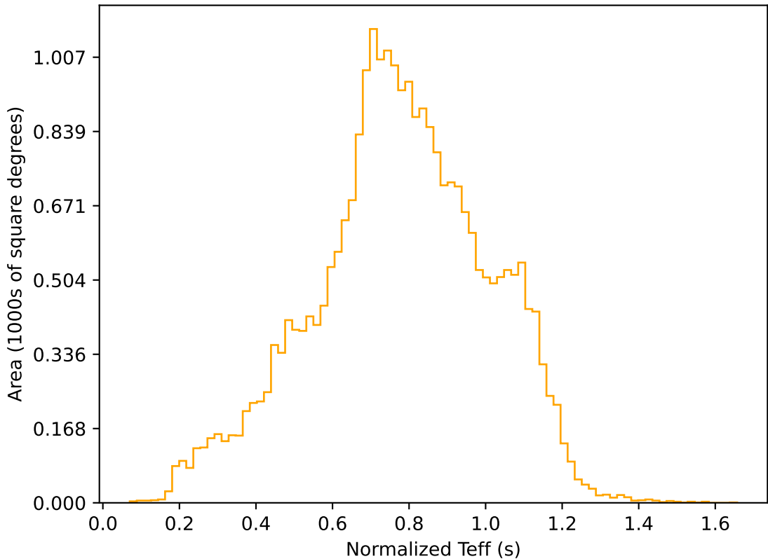
too_elab_r256_d2_ugrizy_v3.4_10yrs All sky r band: Normalized Teff
