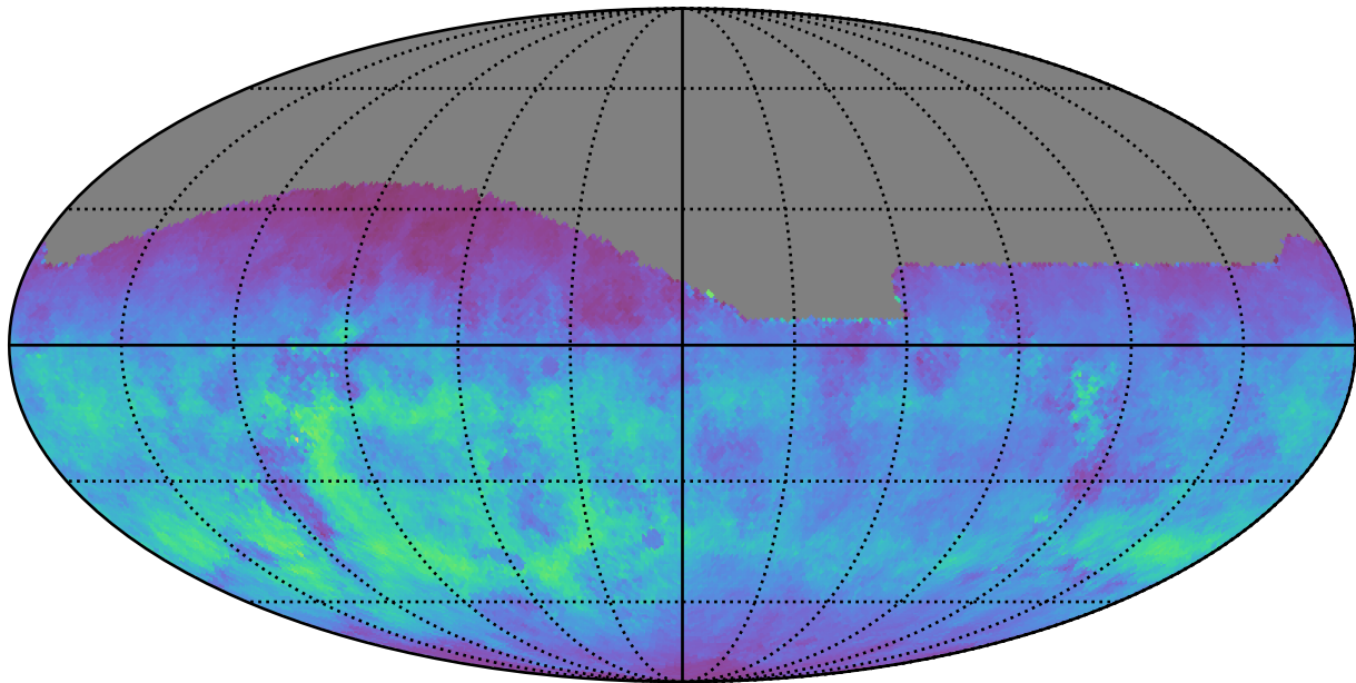
too_elab_r256_d2_ugrizy_v3.4_10yrs All sky g band: Normalized Teff
