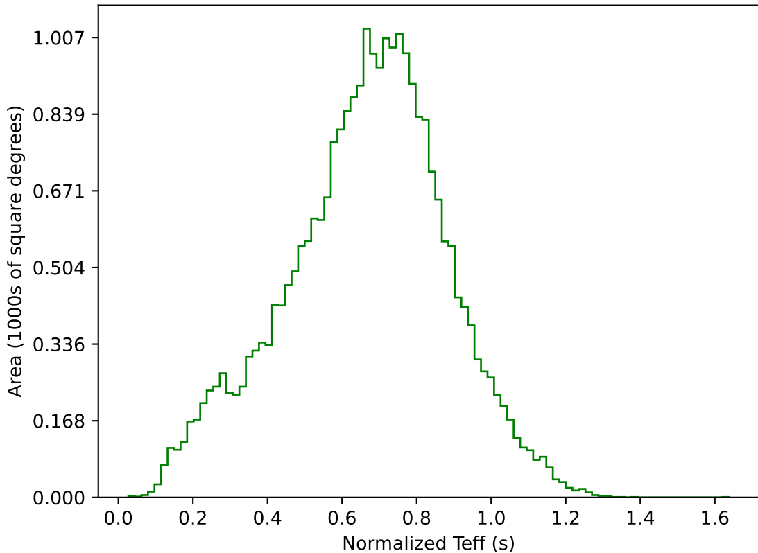
too_elab_r256_d2_ugrizy_v3.4_10yrs All sky g band: Normalized Teff
