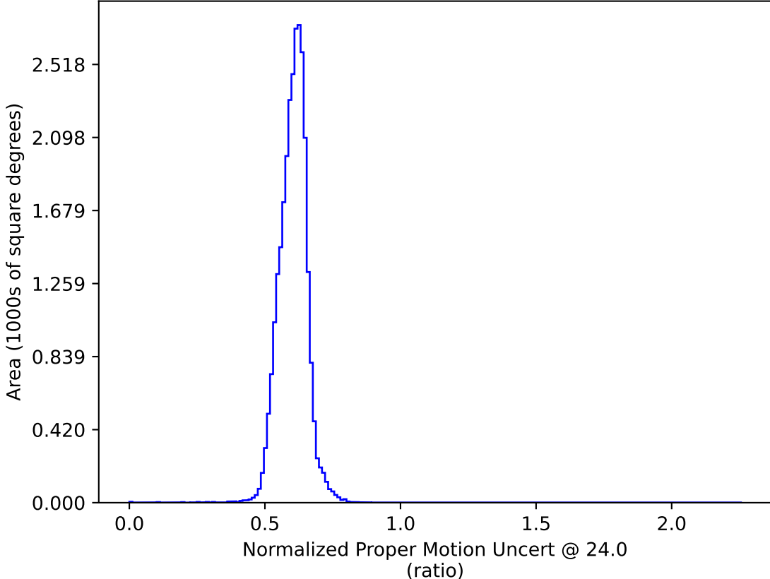
too_elab_r256_d2_ugrizy_v3.4_10yrs All sky: Normalized Proper Motion Uncert @ 24.0
