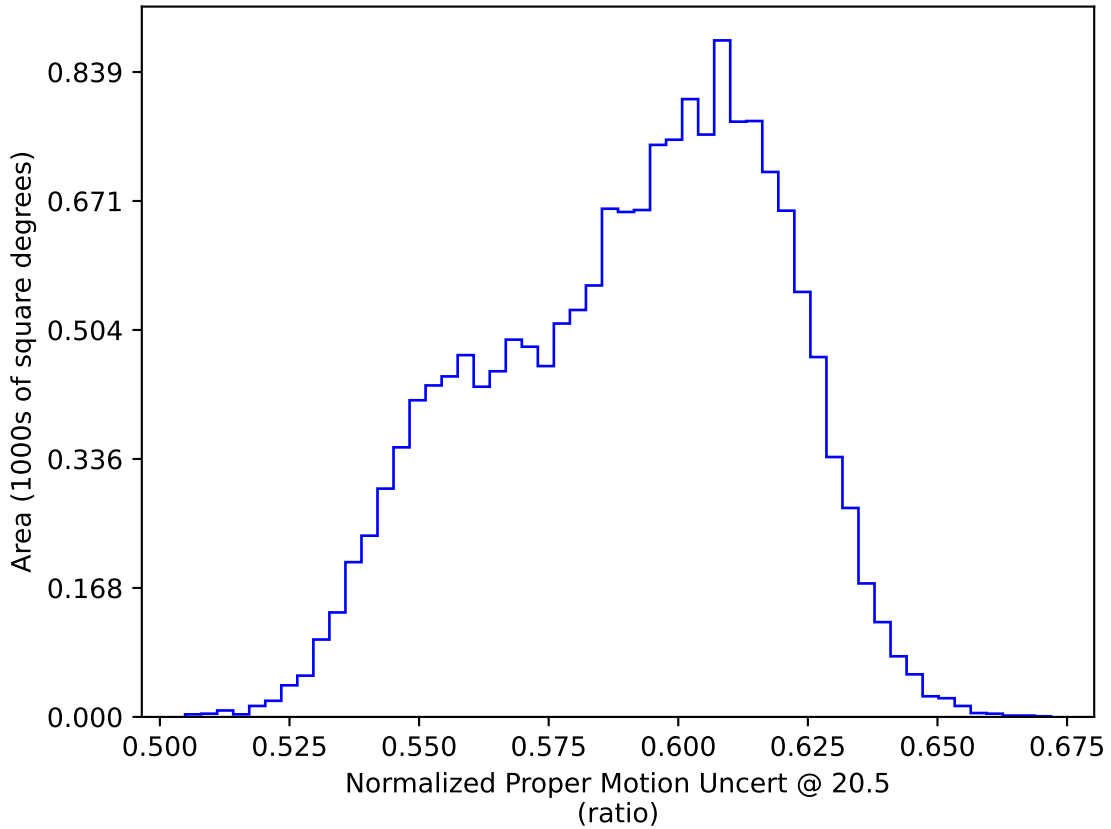
too_elab_r256_d2_ugrizy_v3.4_10yrs WFD: Normalized Proper Motion Uncert @ 20.5
