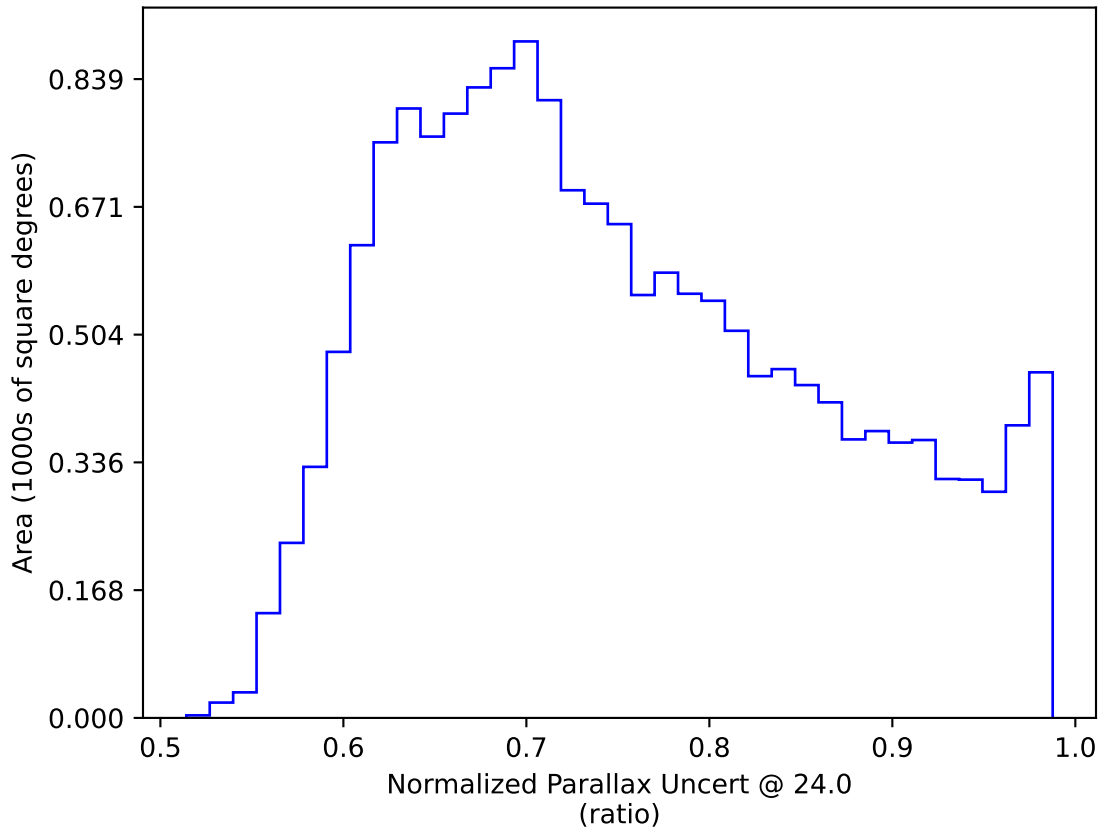
too_elab_r256_d2_ugrizy_v3.4_10yrs WFD: Normalized Parallax Uncert @ 24.0
