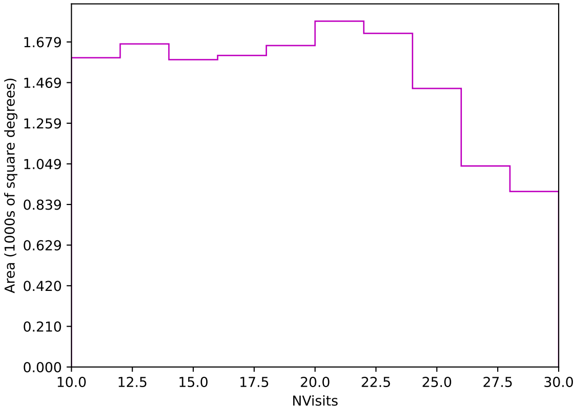
too_elab_r256_d2_ugrizy_v3.4_10yrs Yr 3-4 z band: NVisits
