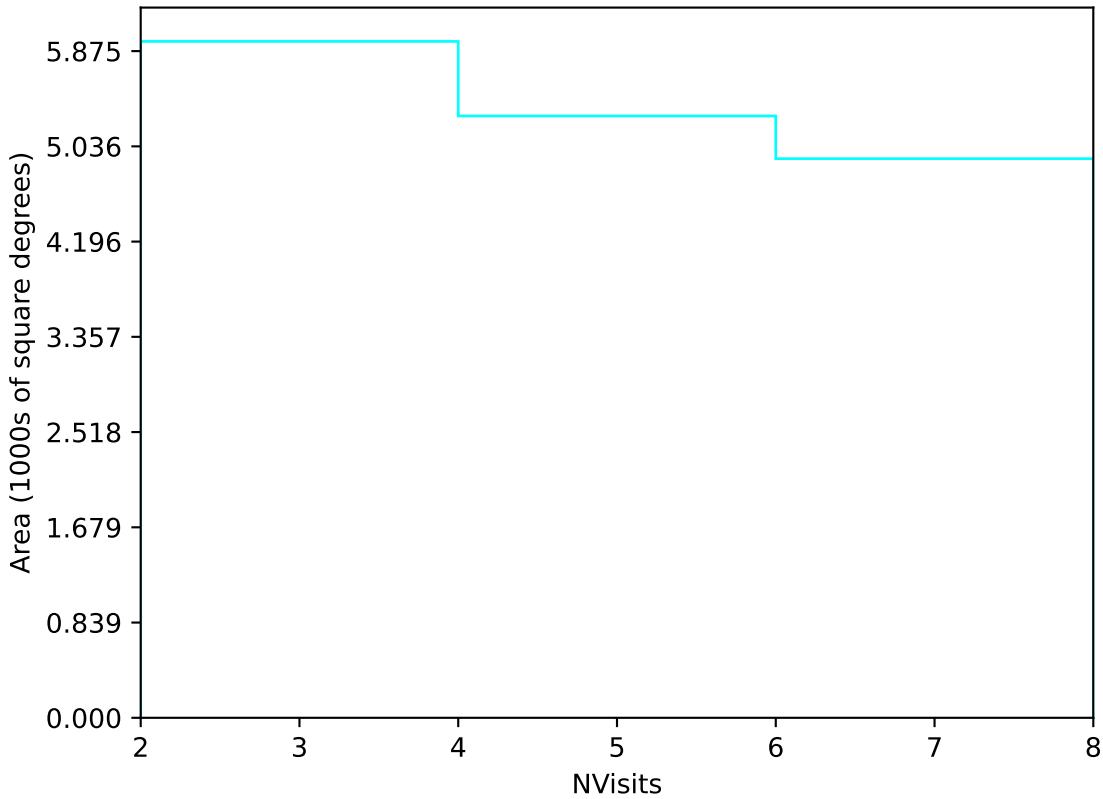
too_elab_r256_d2_ugrizy_v3.4_10yrs Yr 3-4 u band: NVisits
