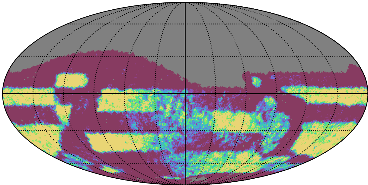
too_elab_r256_d2_ugrizy_v3.4_10yrs Yr 3-4 r band: NVisits
