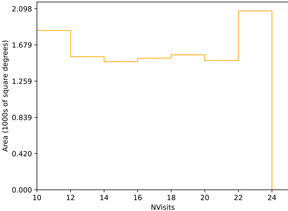
too_elab_r256_d2_ugrizy_v3.4_10yrs Yr 3-4 r band: NVisits
