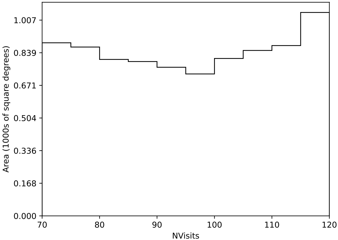
too_elab_r256_d2_ugrizy_v3.4_10yrs Yr 3-4 all bands: NVisits
