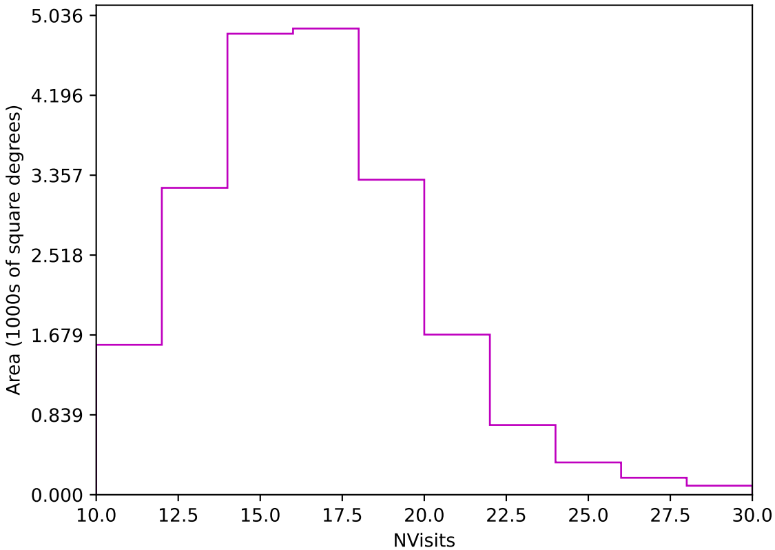
too_elab_r256_d2_ugrizy_v3.4_10yrs Yr 1 z band: NVisits
