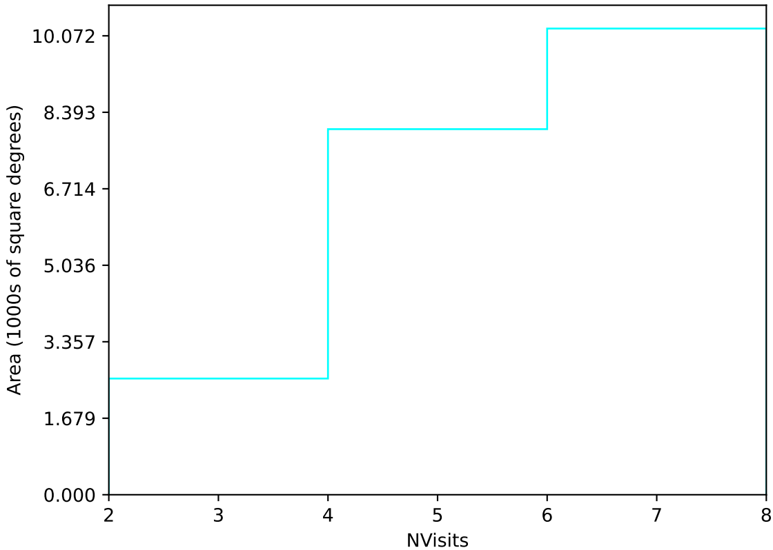
too_elab_r256_d2_ugrizy_v3.4_10yrs Yr 1 u band: NVisits
