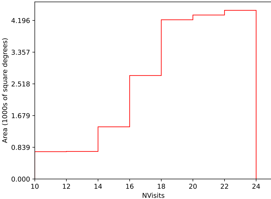
too_elab_r256_d2_ugrizy_v3.4_10yrs Yr 1 i band: NVisits
